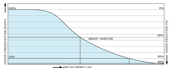
B Shows the result after installing an Aerox®-Injector.
